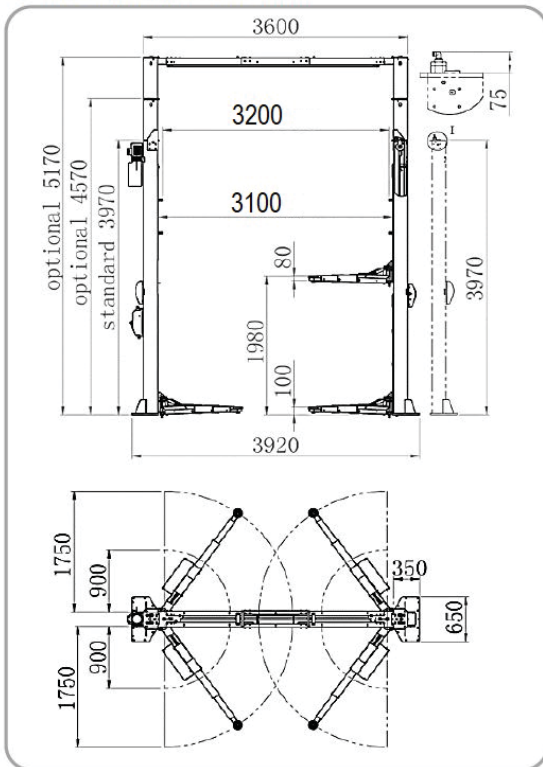
1.2 LAYOUT SYMMETRIC WAY TO INSTALLATION
