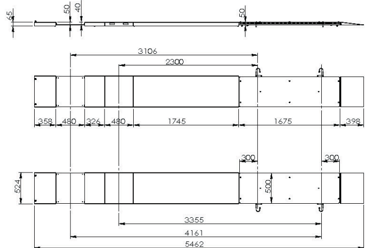
Optional Bolt on Alignment Kit
