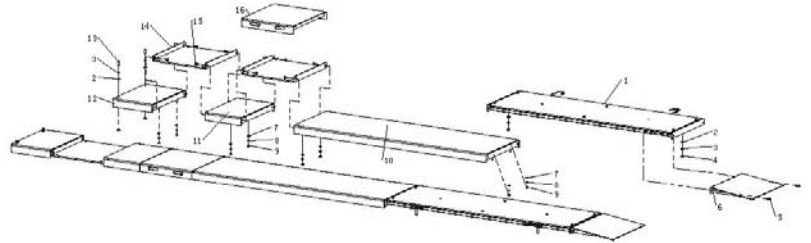
Optional Bolt on Alignment Kit
