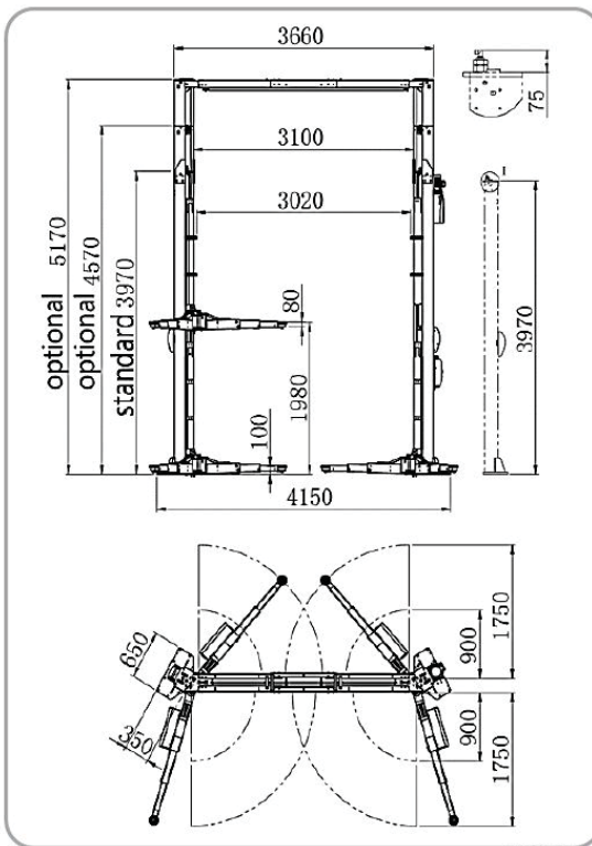
1.21 LAYOUT ASYMMETRIC WAY TO INSTALLATION
